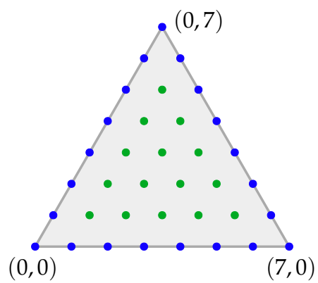
Figure 1: Example of the triangular domain T and numerical grid for the case of n = 7 . The corner points are labeled with their grid indices (i, j) . Blue circles denote the boundary points, and green circles denote the interior points.
